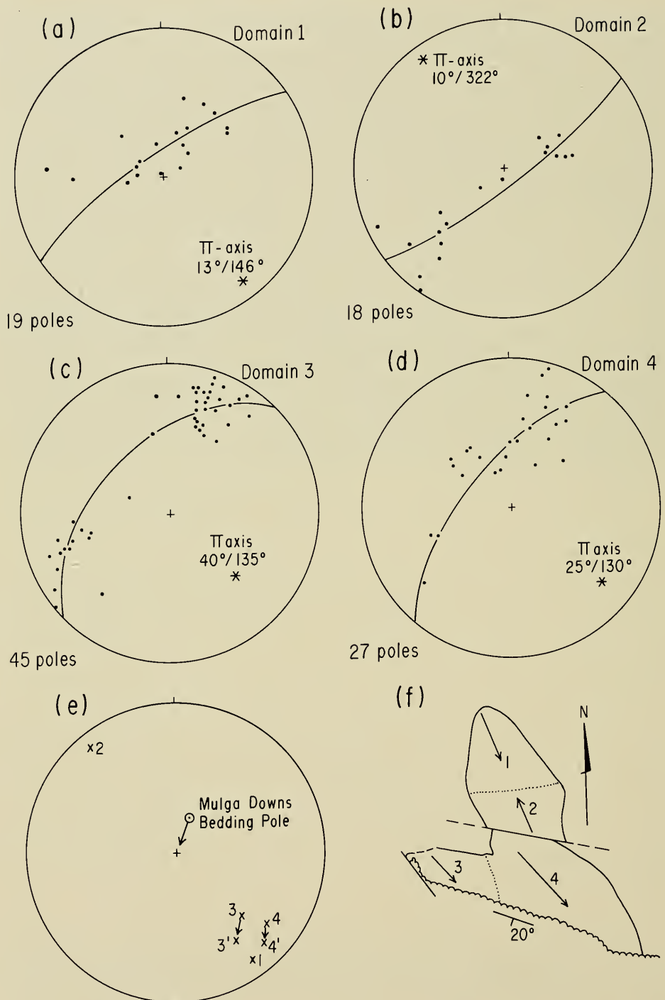
Fig. 6. Equal-area stereograms. (a) to (d) Bedding-pole data from 4 domains in Cupala Creek Formation. (e) Restoration of fold axes in domains 3 and 4 to pre-Mulga Downs Group attitude. (f) Map of domains.
